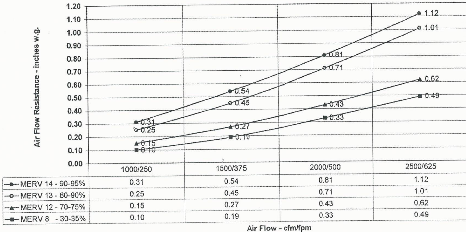
Resistance vs. Air Flow
