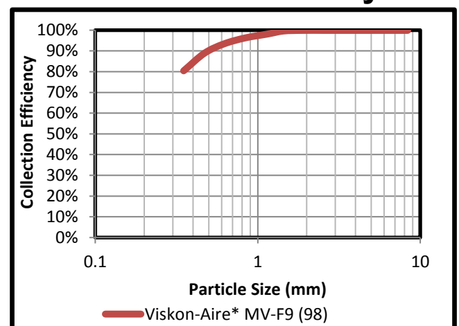
Particle Size Efficiency
